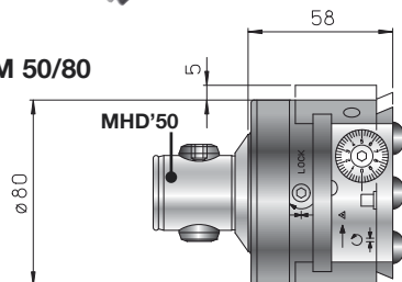
TRM 80/80
