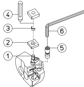
PSRNR/L
